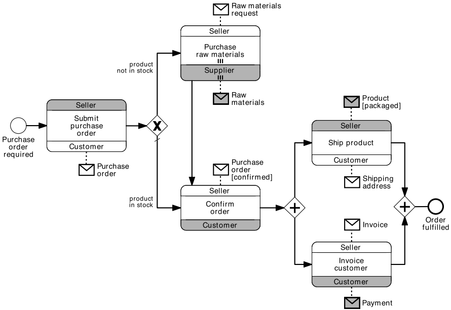
Fig. 4.26 The choreography diagram for the collaboration diagram in Fig. 4.9
