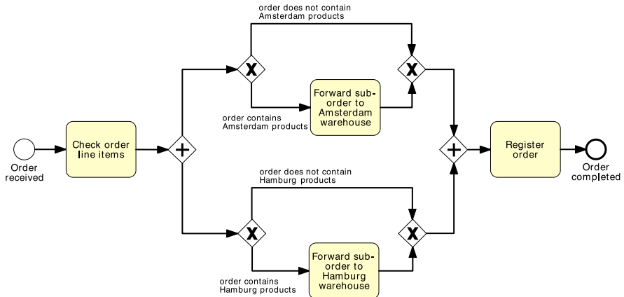
Fig. 3.9 Modeling an inclusive decision: second trial
